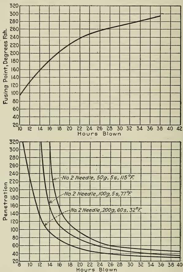
FIG. 110.—Effect of Blowing on the Fusing-Point and Hardness of Petroleum Asphalt.
